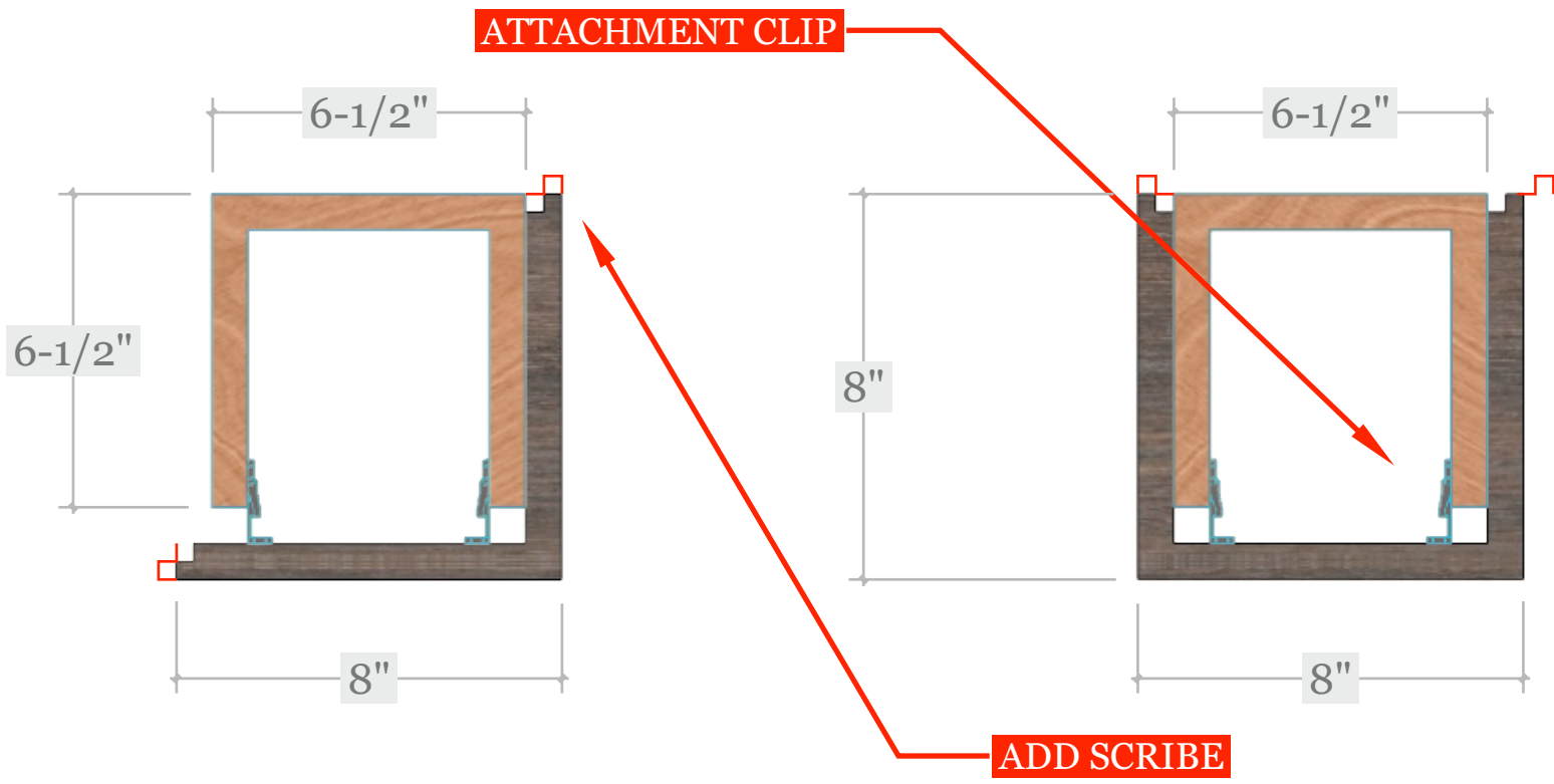
SD D SIDE DETAIL - BEAMS
