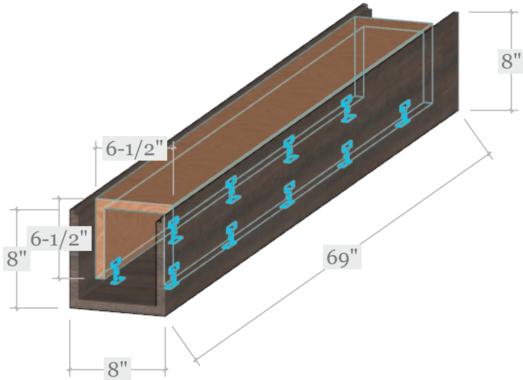
ISO A ISOMETRIC VIEW FULL BEAM
