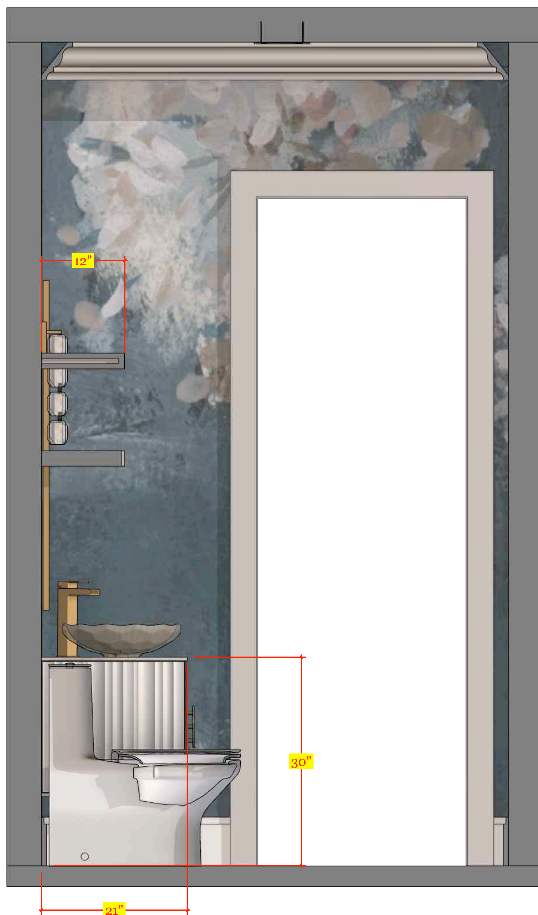
ELV ELEVATION B (SIDE VIEW) B Scale: 1-1/2" = 1'-0"
