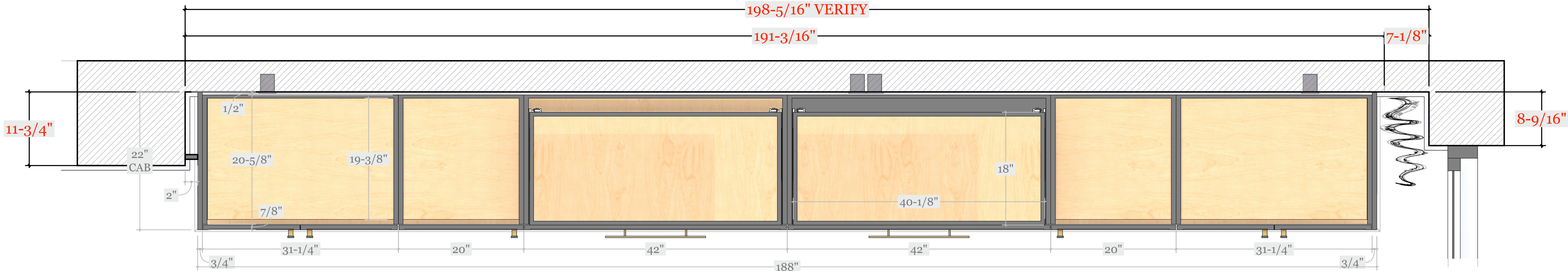
TOP A PLAN VIEW - BOTTOM SECTION
