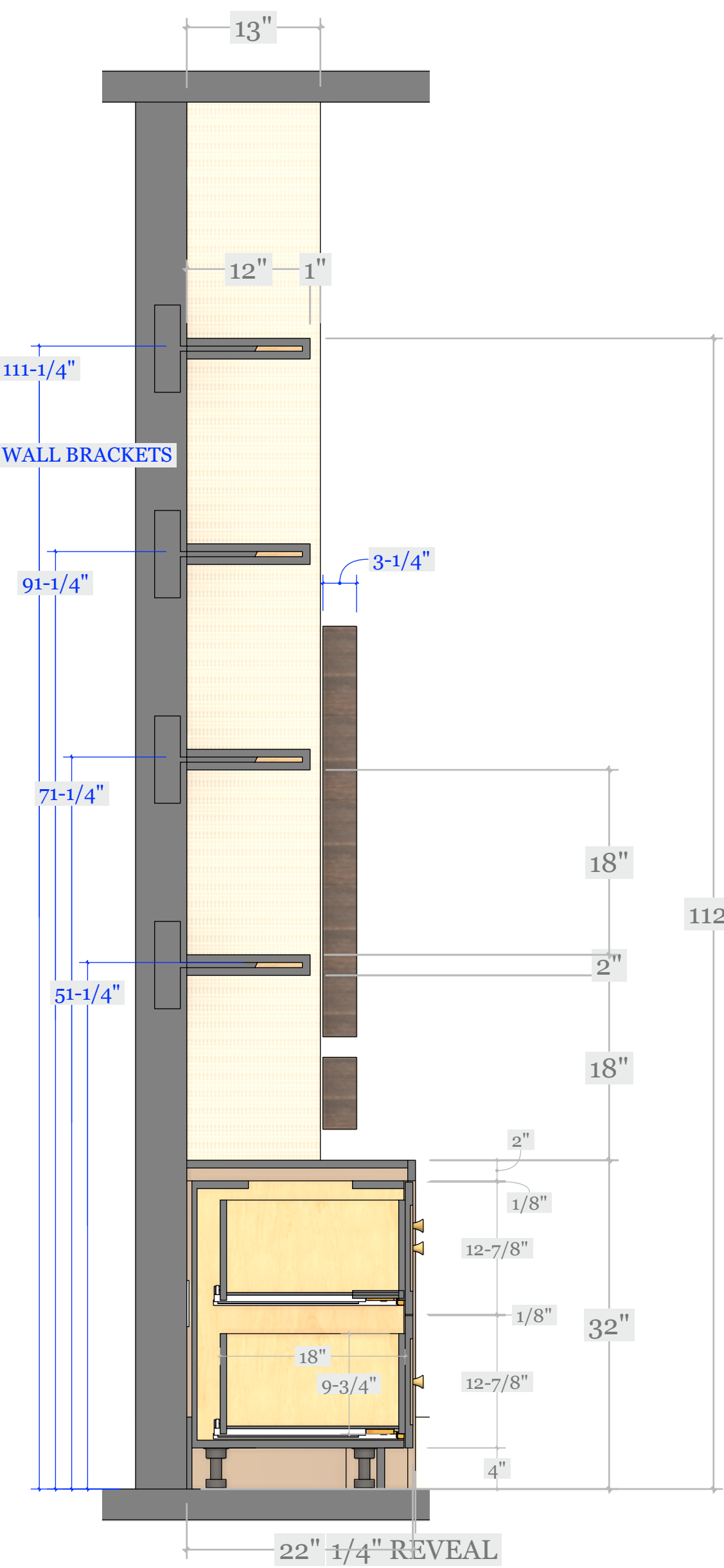
SD A SIDE VIEW - SECTIONS
