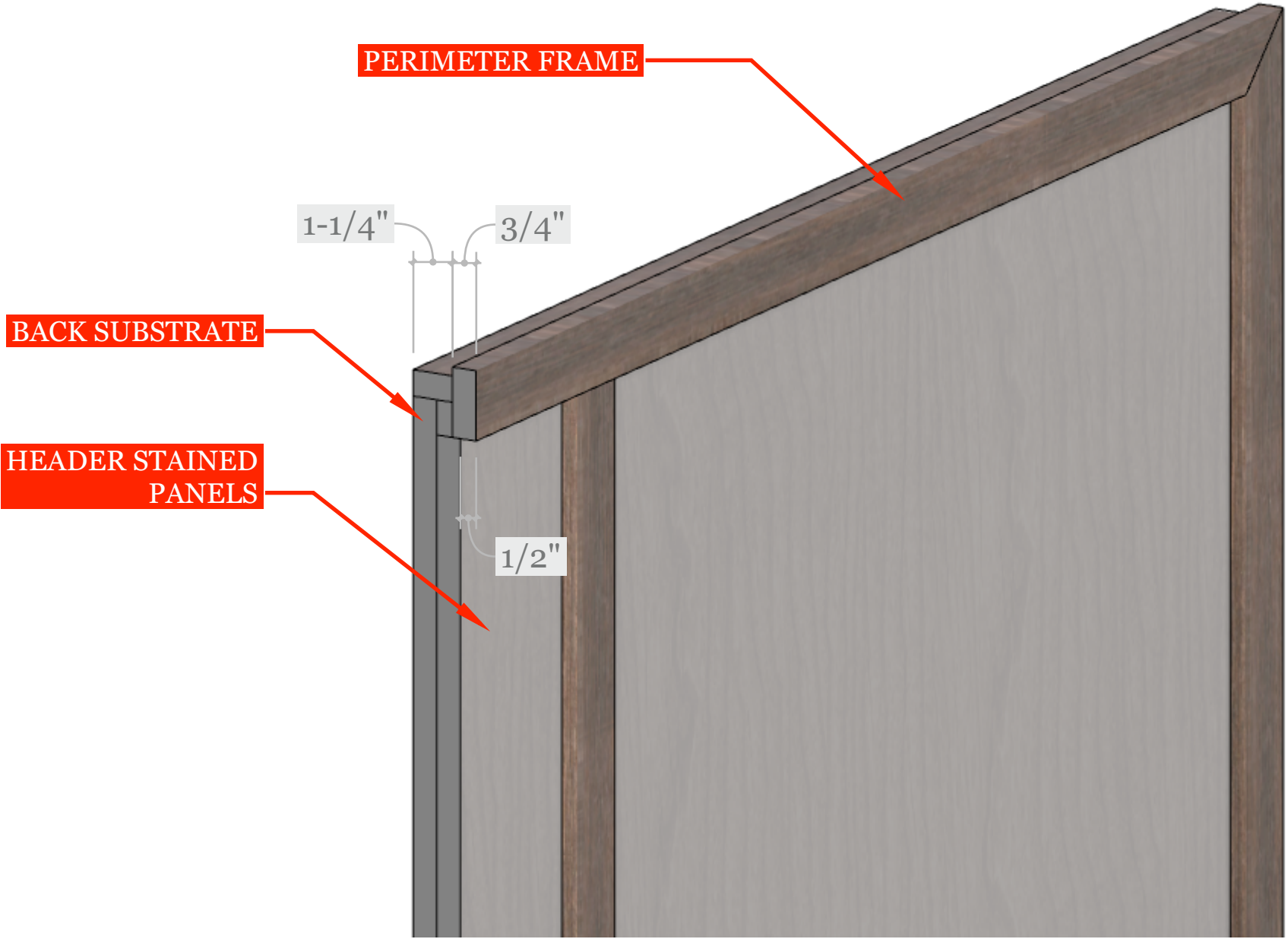
ISO C ISOMETRIC SECTION DETAILS
