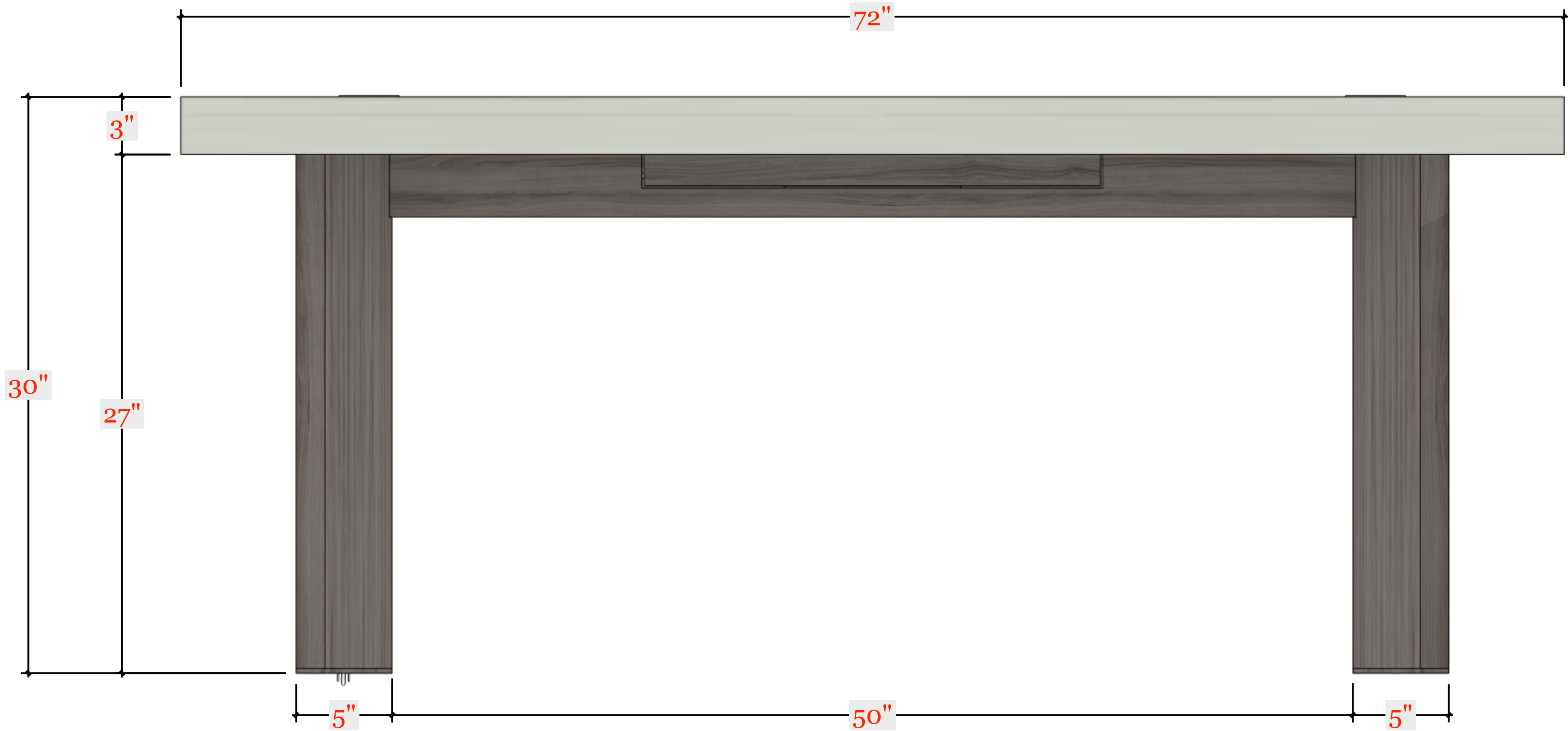
ELV A ELEVATION A
